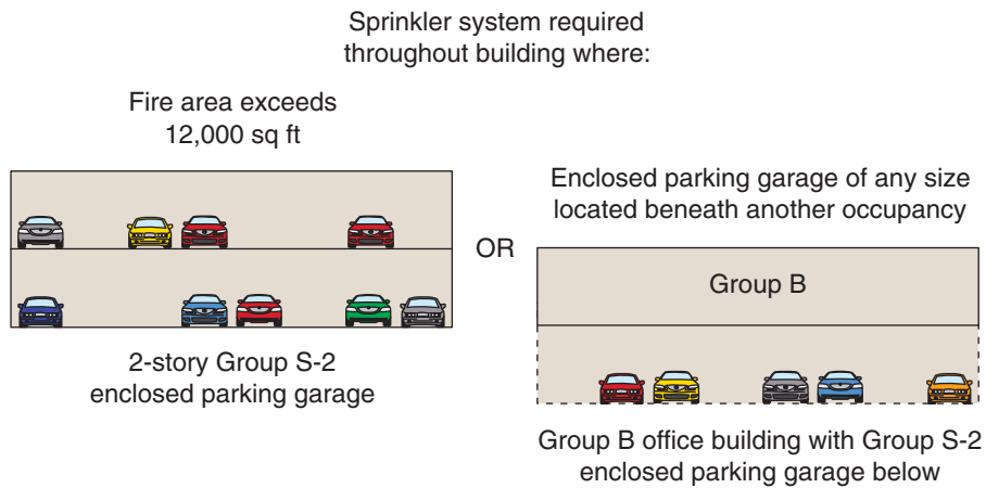
Sprinkler protection of Group S-2 enclosed parking garages
