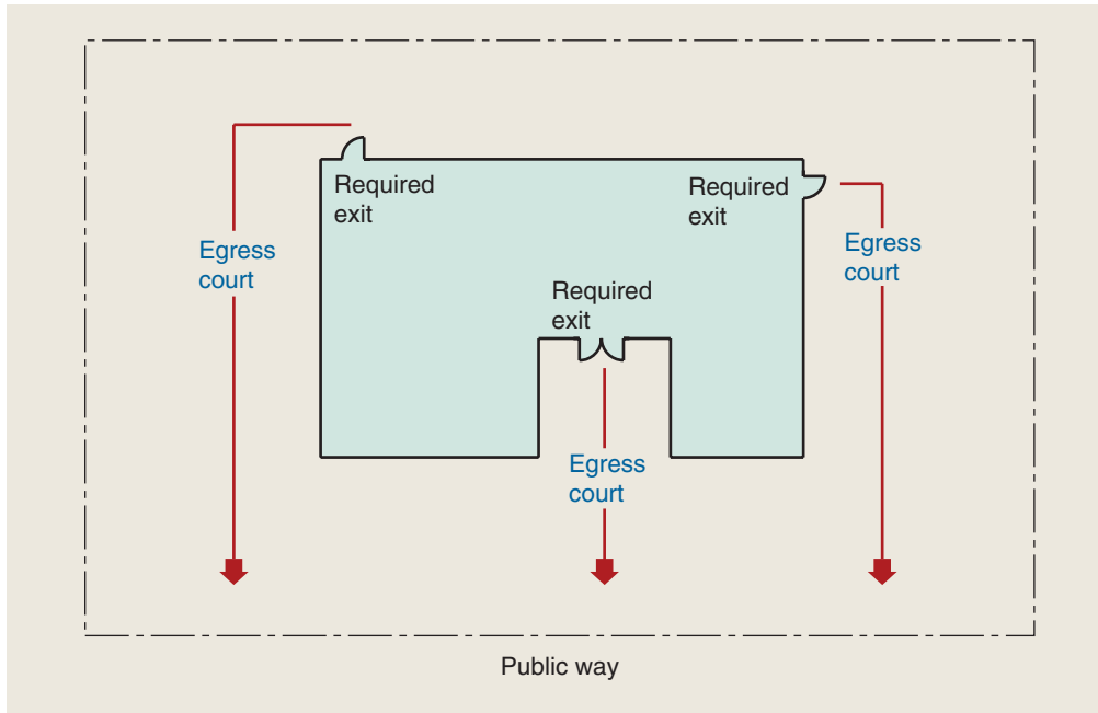
Figure 202-7 Egress court.
